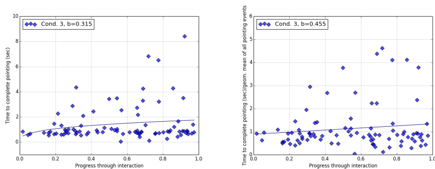
Fig. 7. Results in Condition 3. b_\rho \approx 0.315 , s \approx 1.245 ; b_\mu \approx 0.455
